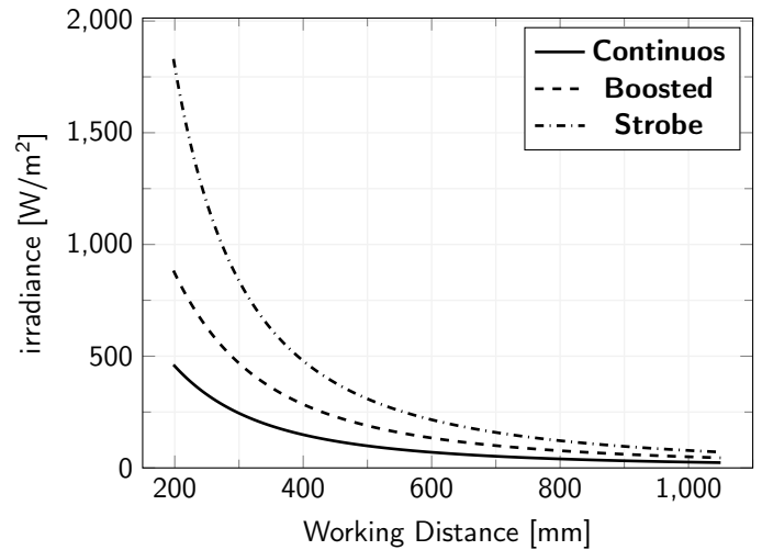
Irradiance Characteristics
